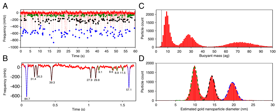
Fig. 3. Buoyant mass measurements of a mixture of 10-, 15-, and 20-nm gold nanoparticles. (A) An arbitrary 60-s oscillation frequency measurement around the resonant frequency of the SNR during a 97-min-long experiment. Data were acquired at 1 kHz and filtered with a five-point second-order Savitzky-Golay filter and a second-order IIR high-pass filter with 1-Hz cutoff frequency. Particles detected by the bank of matched filters ( Methods ) are marked with circles color-coded with respect to their buoyant masses (green for <18 ag, blue for >44 ag, black for in between). (B) Each detected peak is further analyzed for estimating the buoyant mass and the transit time of the particle by fitting it to the expected peak shape for a particle transiting the cantilever with a constant velocity. Estimated buoyant mass value for each detected particle is indicated underneath the peak along with the estimated color-coded peak shape. (C) Buoyant mass histogram of 29,000 particles detected during the experiment. The thin dotted line at \sim 5 ag is the limit of mass detection in the experiment. (D) Diameter histogram, calculated assuming particles are uniform spheres of density 19.3 g/cm 3 . Dashed lines show fits to Gaussians. Particle peaks shown in A and B belong to the corresponding populations in D with the matching color. The fits indicate mean sizes of 9.9, 14.4, and 19.7 nm with coefficients of variation of 7.4%, 5.3%, and 4.9%, respectively.
